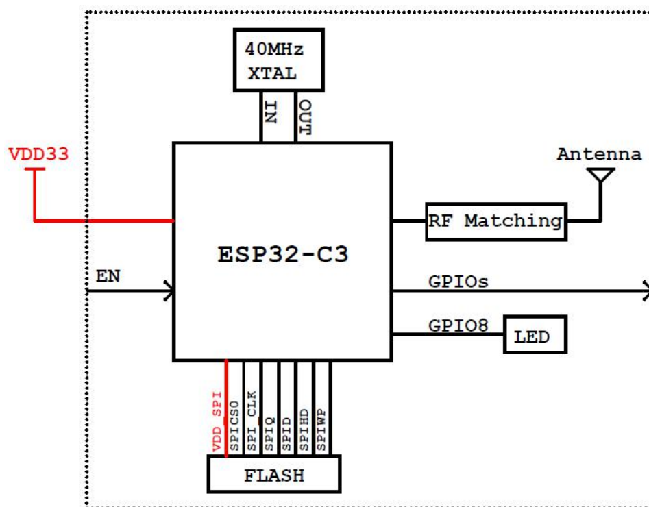
Figure 1 Block diagram
