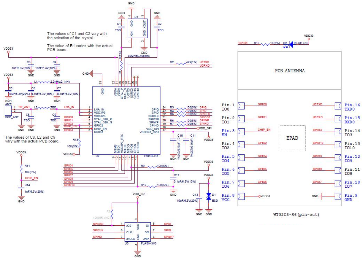
Figure 6 Module schematics
